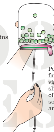
Fig. 1.10: A model for happy converting of solid to liquid and liquid to gas.
